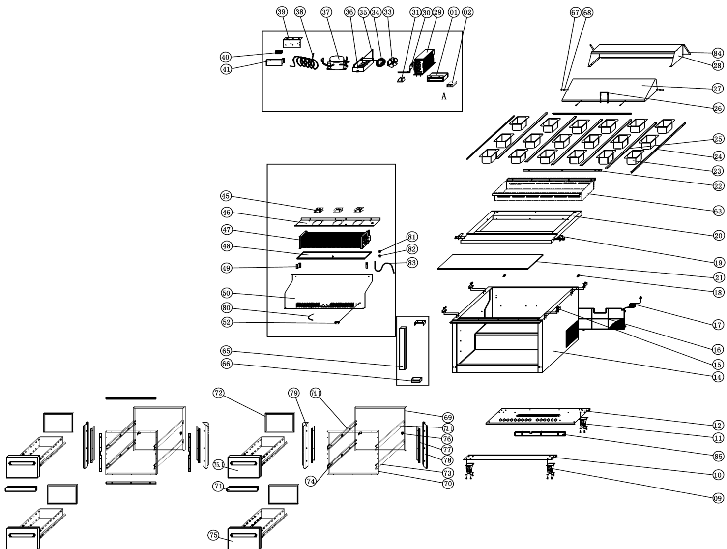
EXPLODE OF KCHMT48.18.4D
